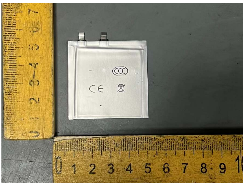
Figure 2 Overall view 2 of cell (电芯外观图2)
